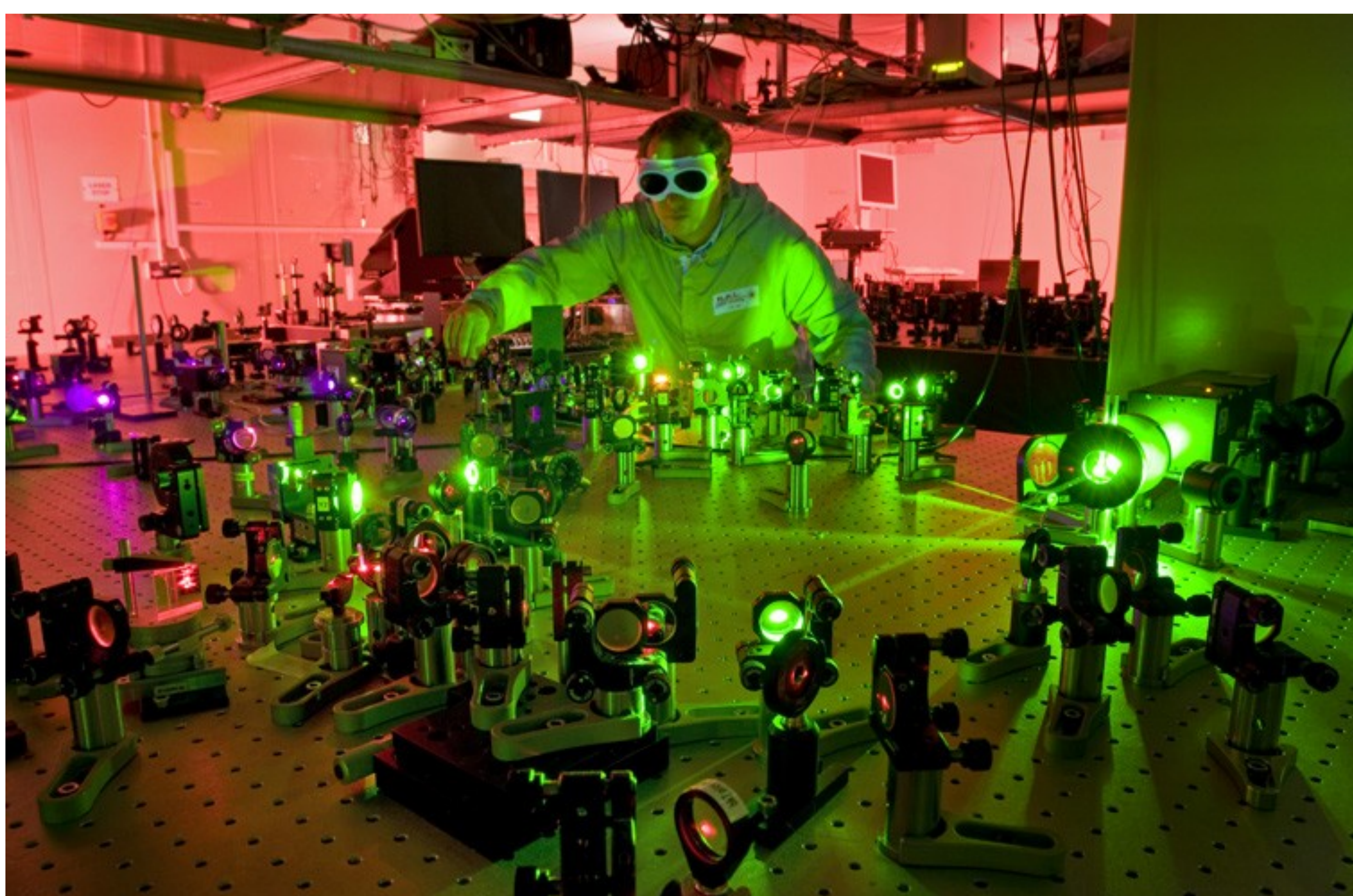
Figure 2. Photograph of the laboratory housing the prototype front-end oscillator and the initial OPCPA amplifier stages for the 10 PW proposal.
