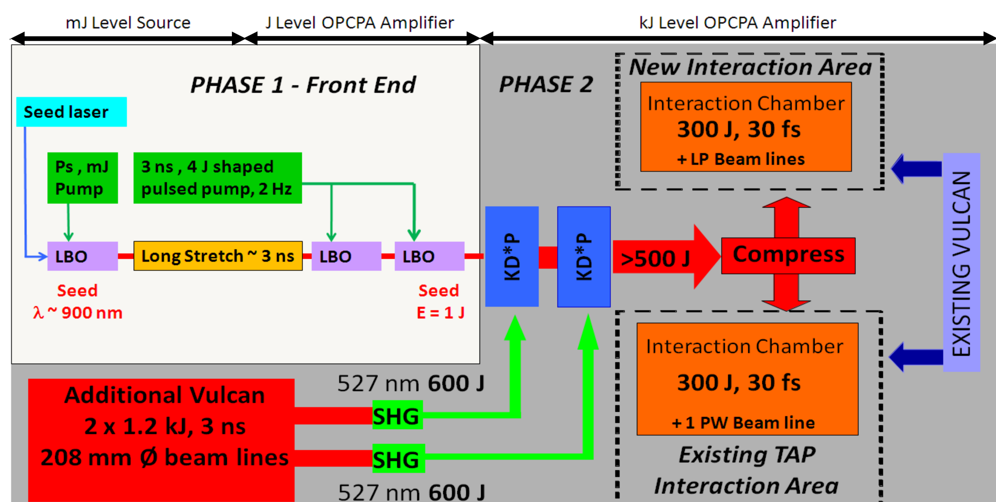
Figure 3. Schematic of the new OPCPA front end oscillator built as an initial proof-of-principle and how it will be integrated into the full system to be built in Phase 2.
